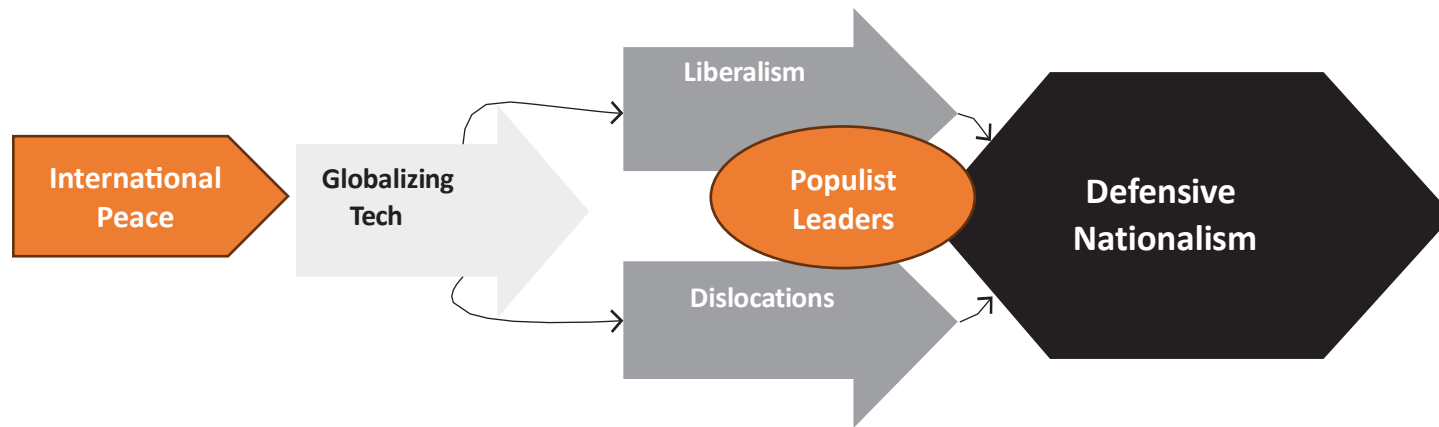
Figure 1: Logic of the Argument
